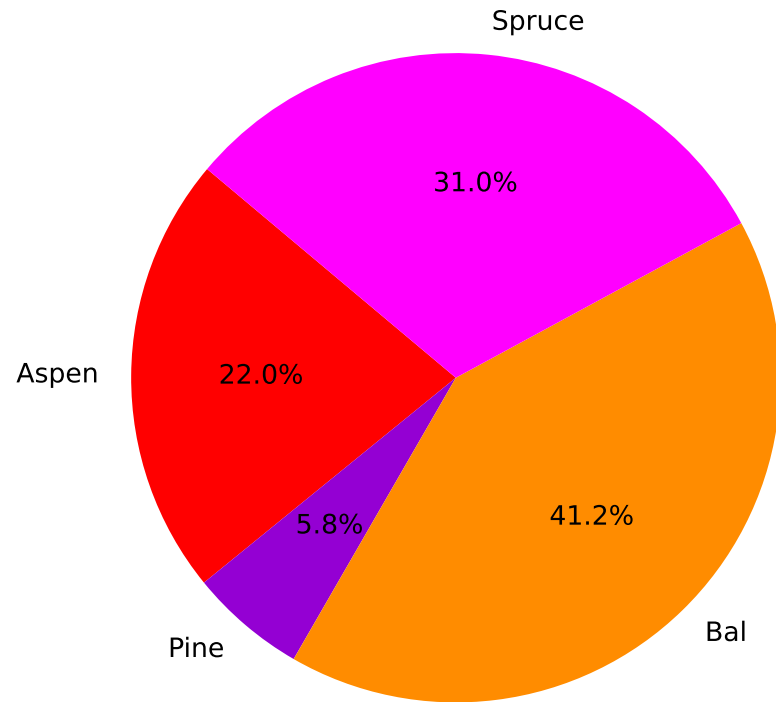
Species Distribution at Time Period 0
